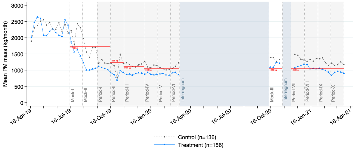
Figure 6: PM emissions by treatment status
