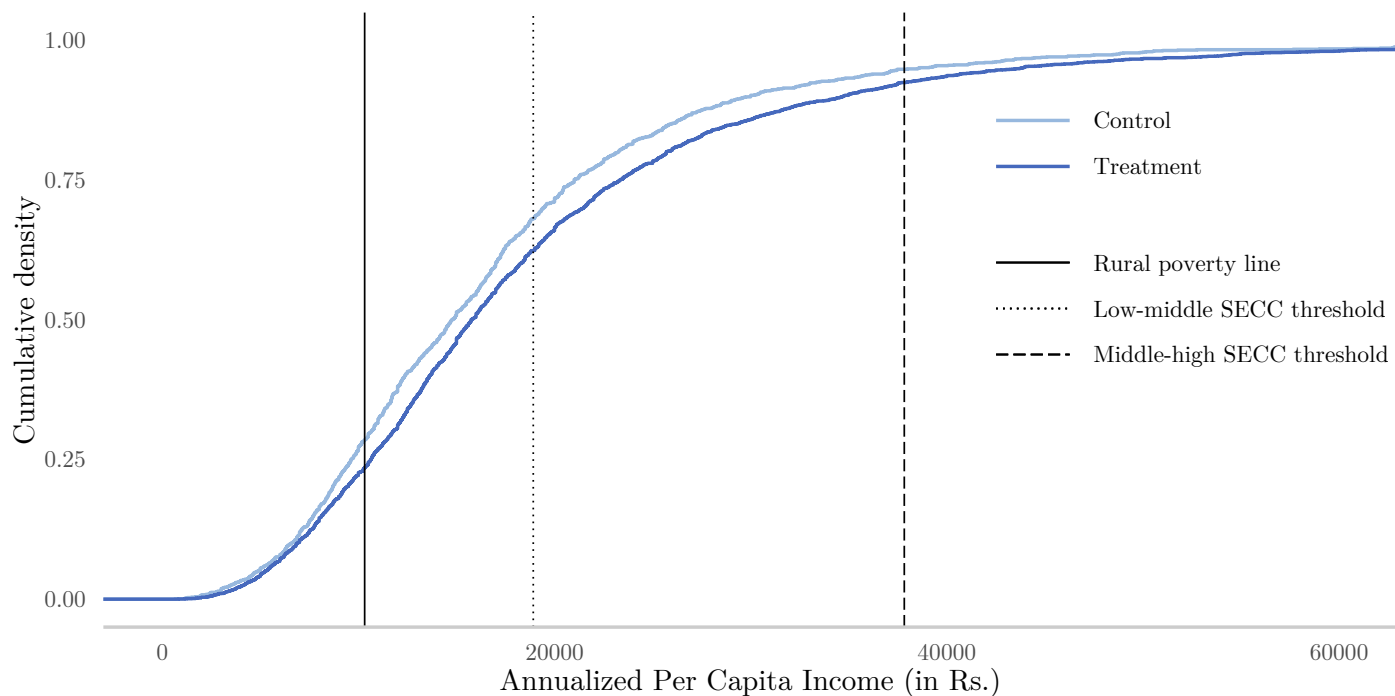
Figure A.3: Income distribution by treatment status
